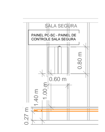
2 VISTA FRONTAL PC-SC 1:50
