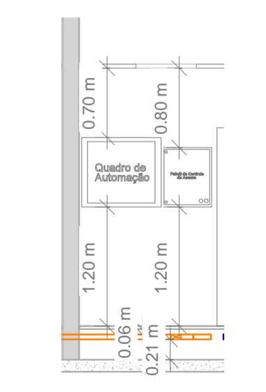
3 VISTA FRONTAL QC-AUT-01 1:50
